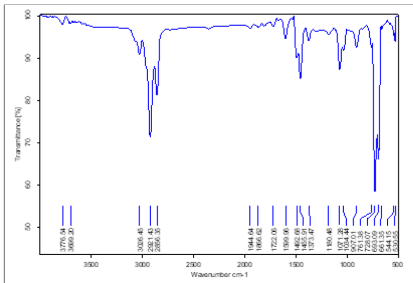
Fig 12: FTIR analyses for the SEBS solution (High concentration) in THF at the ratio 20:80
