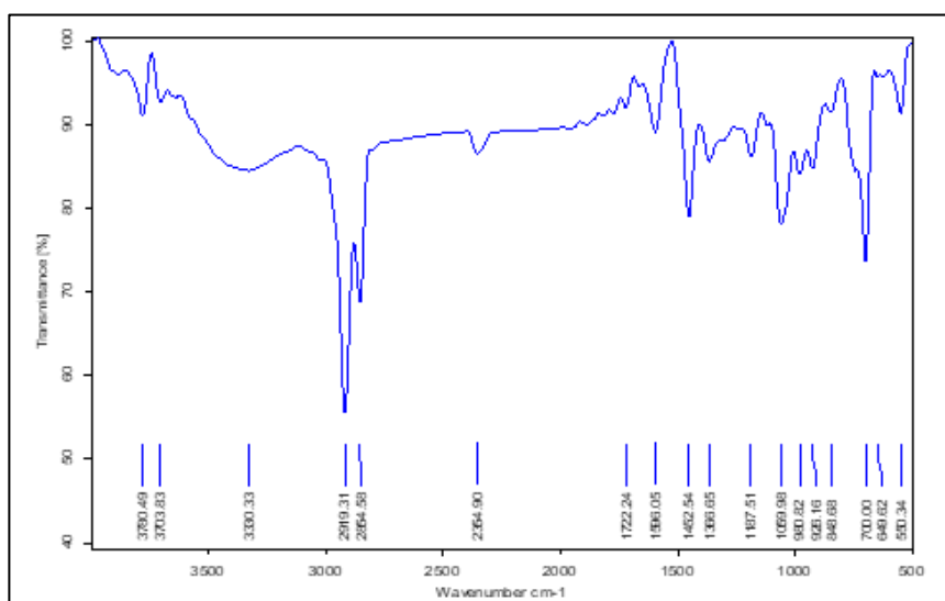
Fig 7: FTIR analyses for the SEBS solution (Low concentration) in THF at the ratio 40:60
