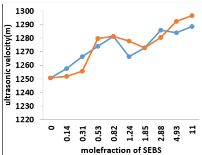
Fig 2: Variation of ultrasonic velocity with Mole fraction of SEBS in Tetrahydrofuran solution in low and high concentration at 303K
