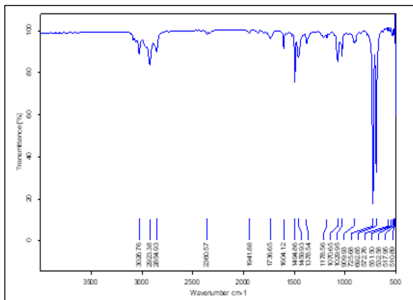
Fig 9: FTIR analysis for the SEBS solution (High concentration) in THF at the ratio 90:10
