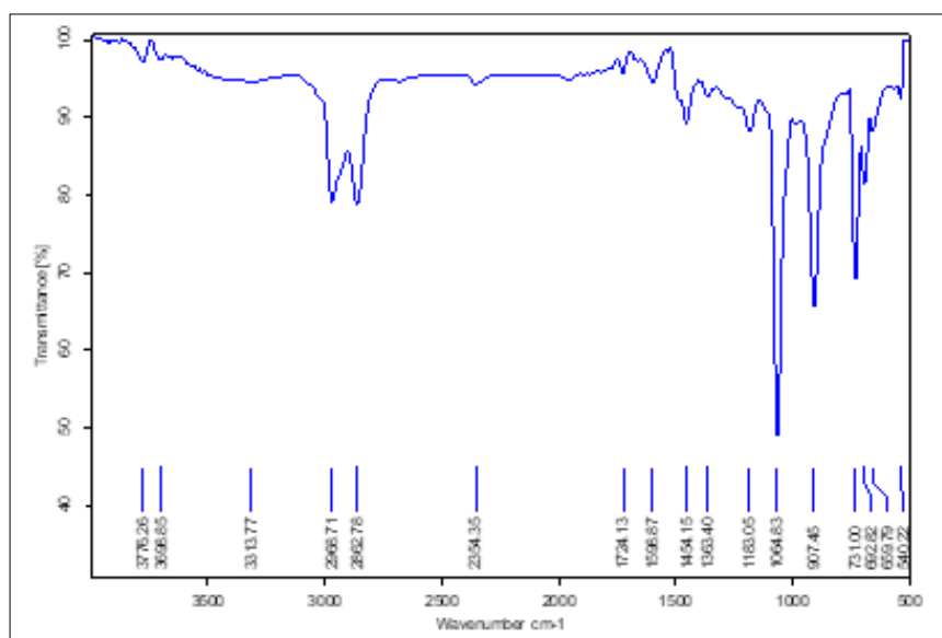
Fig 8: FTIR analyses for the SEBS solution (Low concentration) in THF at the ratio 10:90
