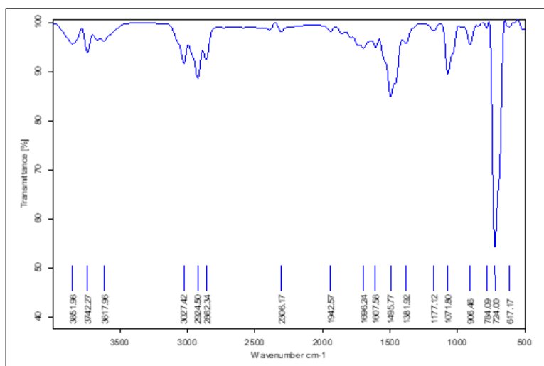
Fig 5: FTIR analyses for the SEBS solution (Low concentration) in THF at the ratio 90:10
