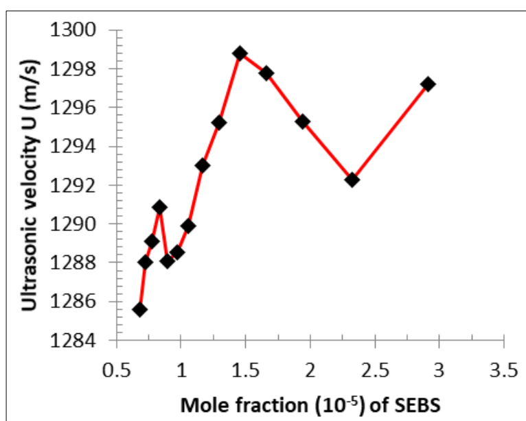
Fig 1: Variation of ultrasonic velocity with mole Fraction of SEBS in toluene solution
