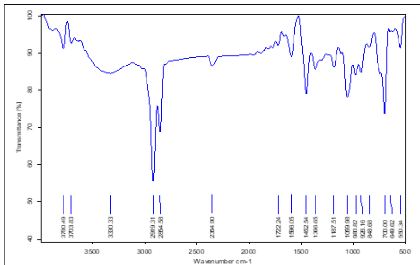
Fig 6: FTIR analyses for the SEBS solution (Low concentration) in THF at the ratio 30:70
