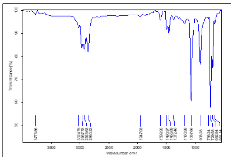
Fig 11: FTIR analyses for the SEBS solution (High concentration) in THF at the ratio 40:60
