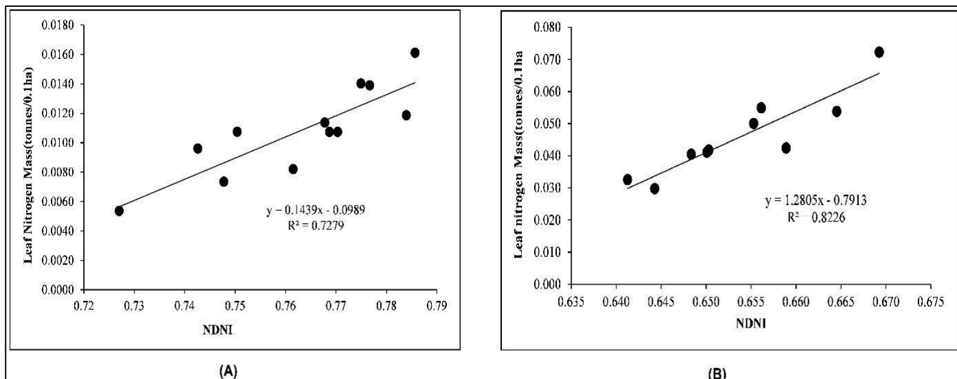
Fig 4: Regression plot between NDNI and Leaf Nitrogen Mass for (A) Sal and (B) Oak
