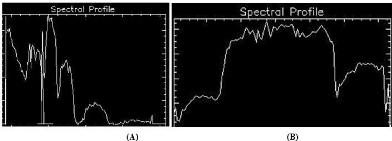
Fig 3: Spectral profile before (A) and after (B) atmospheric correction
