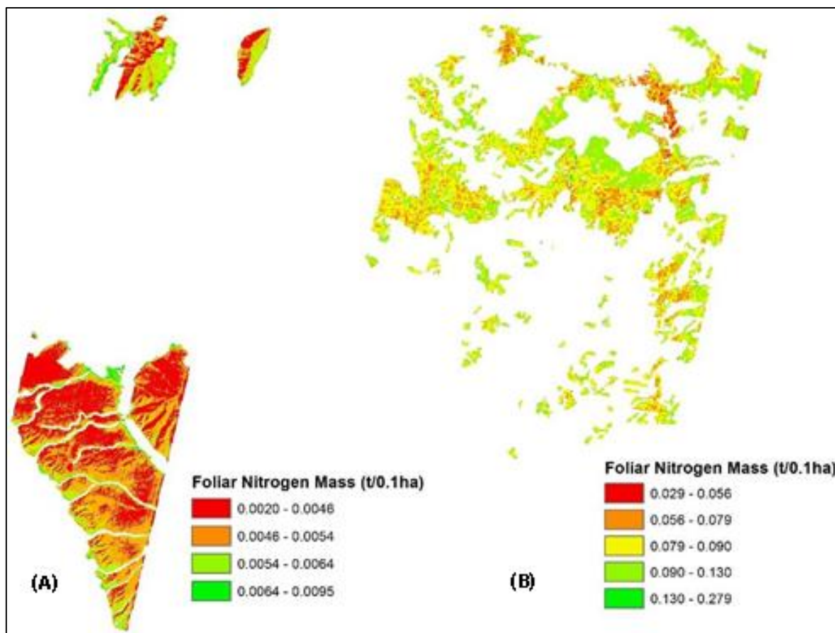
Fig 5: Foliar nitrogen mass map of (A) Sal and (B) oak vegetation
