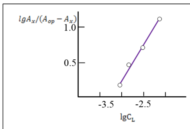
Fig 4: Determination of the ratio of components by equilibrium shift method for Cu - MPAMPT C_{Cu} = 1.875 \times 10^{-5} M ; C_{MPAMPT} = 5.0 \times 10^{-4} M , pH=6, \lambda = 590 \text{ nm} , KFK-2. l = 1 \text{ cm} .
