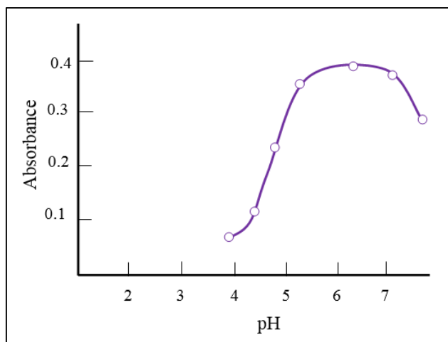
Fig 1: Absorbance of mixed-ligand complexes as a function of the pH of the aqueous phase C_{Cu} = 1.875 \times 10^{-5} M ; C_{MPAMPT} = 5.0 \times 10^{-4} M , KFK-2, \lambda = 590 \text{ nm} , l = 0.5 \text{ cm}
