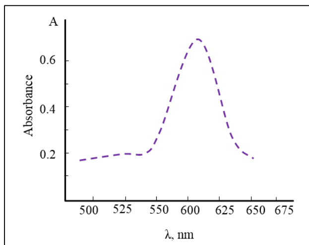
Fig 2: Absorption of complex Cu – MPAMPT C_{Cu} = 1.875 \times 10^{-5} M ; C_{MPAMPT} = 5.0 \times 10^{-4} M , Shimadzu UV1240, l = 1 \text{ cm} .
