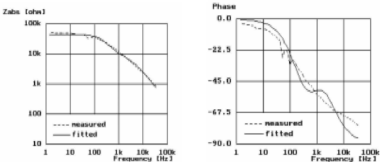
Fig 2: The amplitude and phase diagrams of the Cd 4 GeSe 6 and 0.05 M H 2 SO 4
