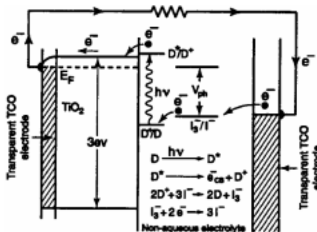
Fig 1: The band diagram of the dyesensitized photoelectrochemical solar cell
