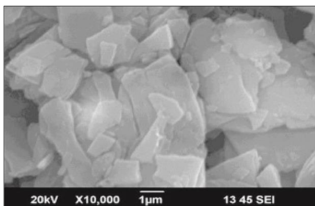
Fig 10: SEM Image of PoPDA with 50mM SDS
