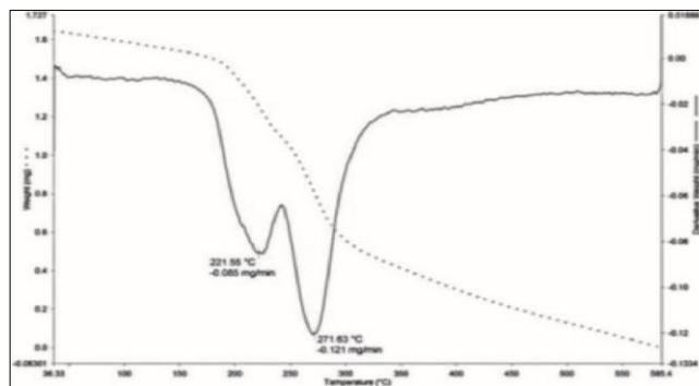
Fig 6: TGA/DTG Thermogram of PoPDA with 50mM SDS
