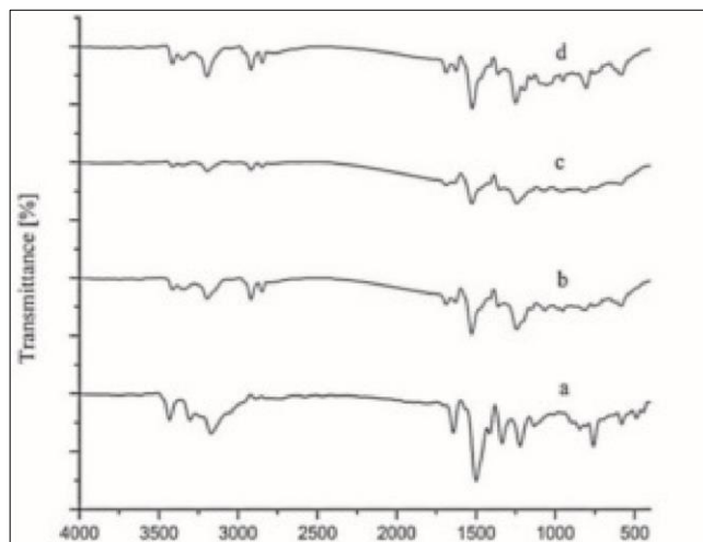
Fig 1: FT-IR Spectrum of PoPDA and PoPDA with Different Concentration of SDS
