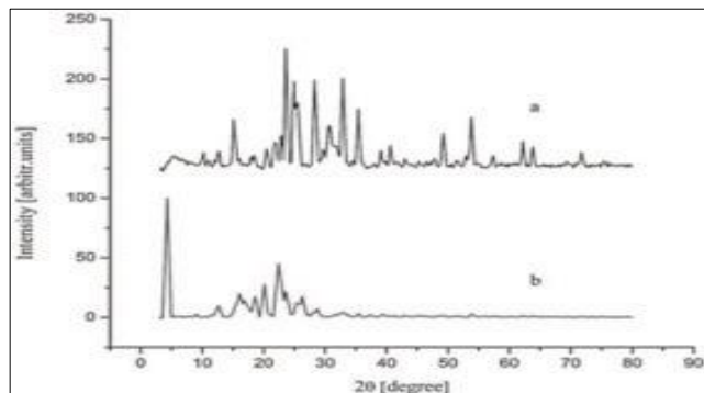
Fig 7: XRD Pattern for PoPDA and PoPDA with SDS at its CMC Backbone
