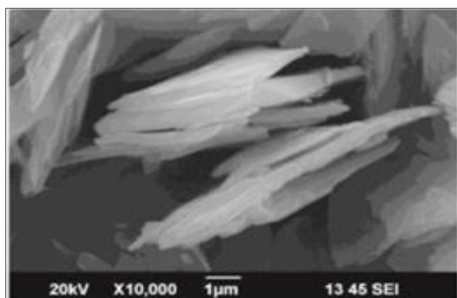
Fig 9: SEM image of PoPDA with 8 mm SDS
