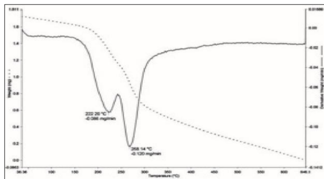
Fig 4: TGA/DTG Thermogram of PoPDA with 5mM SDS
