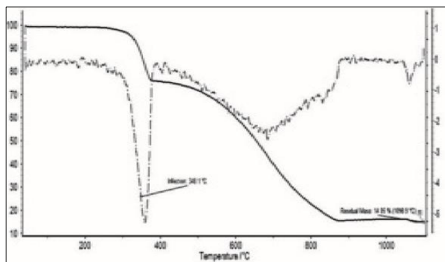
Fig 3: TGA/DTG Thermogram of PoPDA
