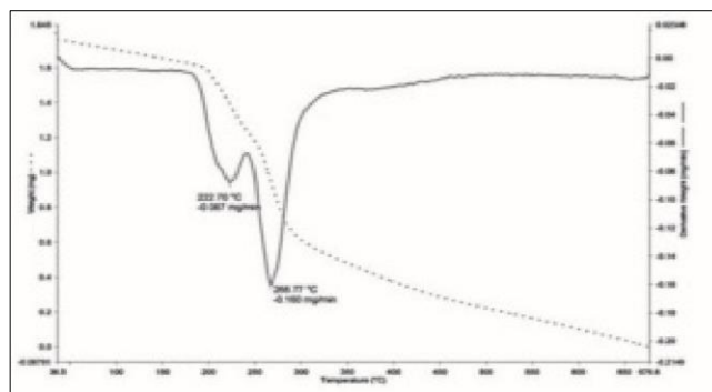
Fig 5: TGA/DTG Thermogram of PoPDA with 8 mM SDS
