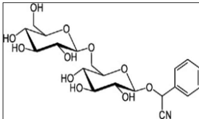
Fig 2: Structure of Laetrole
