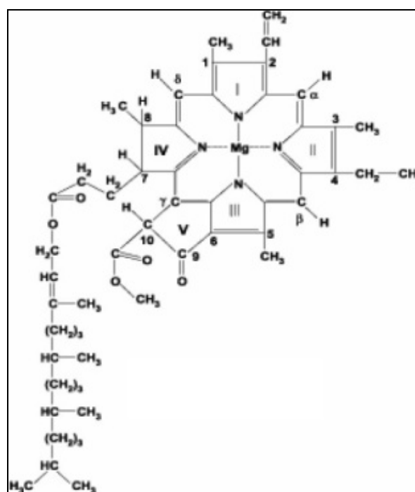
Fig 3: Structure of Chlorophyll Molecules
