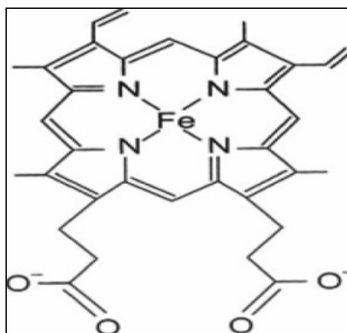
Fig 4: Structure of Tetra Pyrrole Head of Hemoglobin
