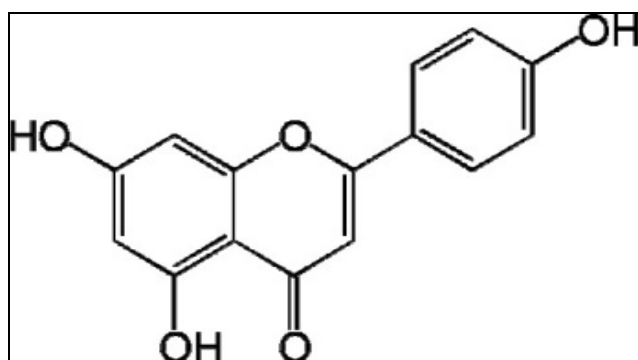
Fig 1: Structure of Apigenin
